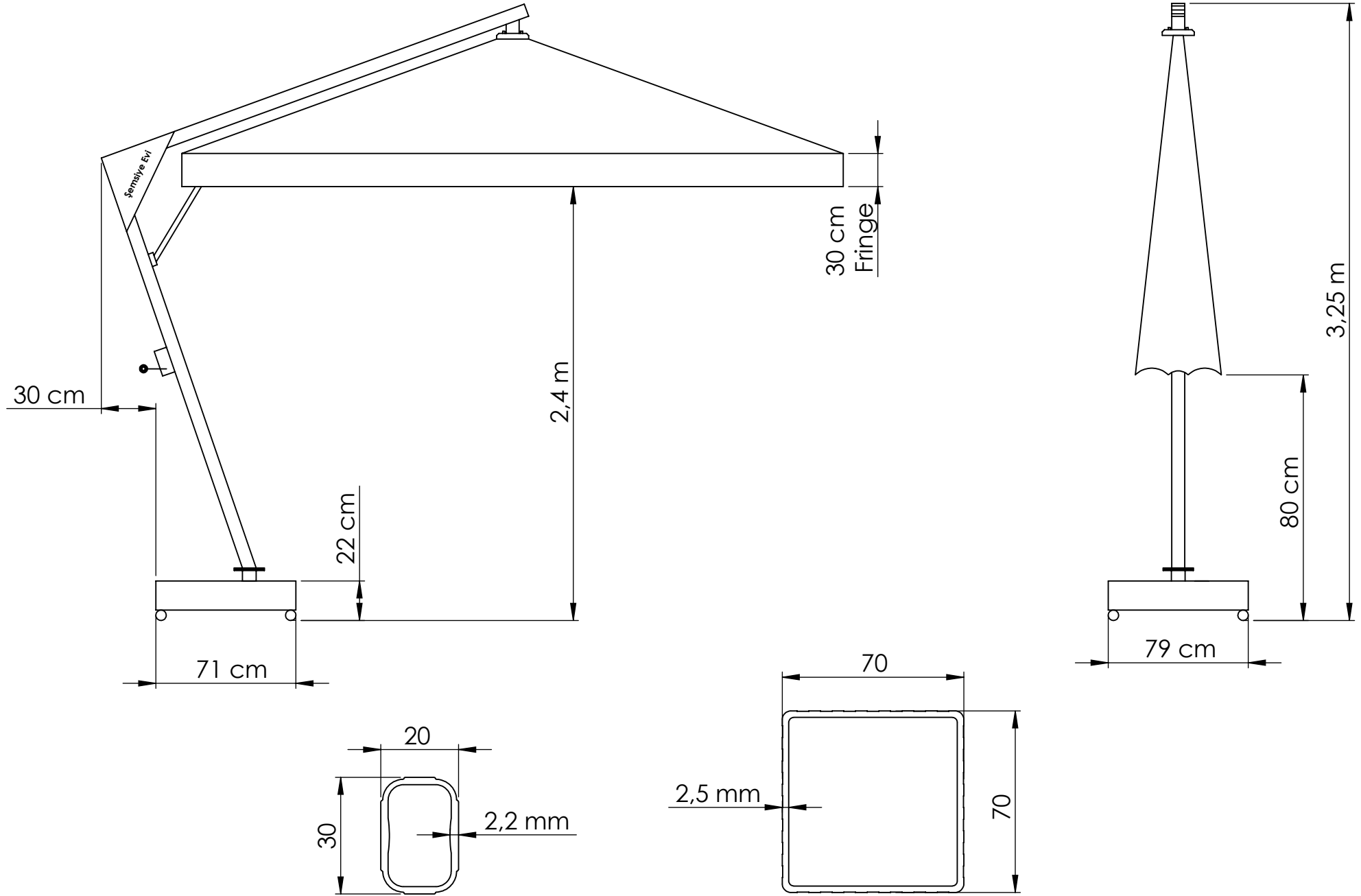
Profil / Ribs
