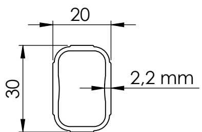
Profil / Ribs
