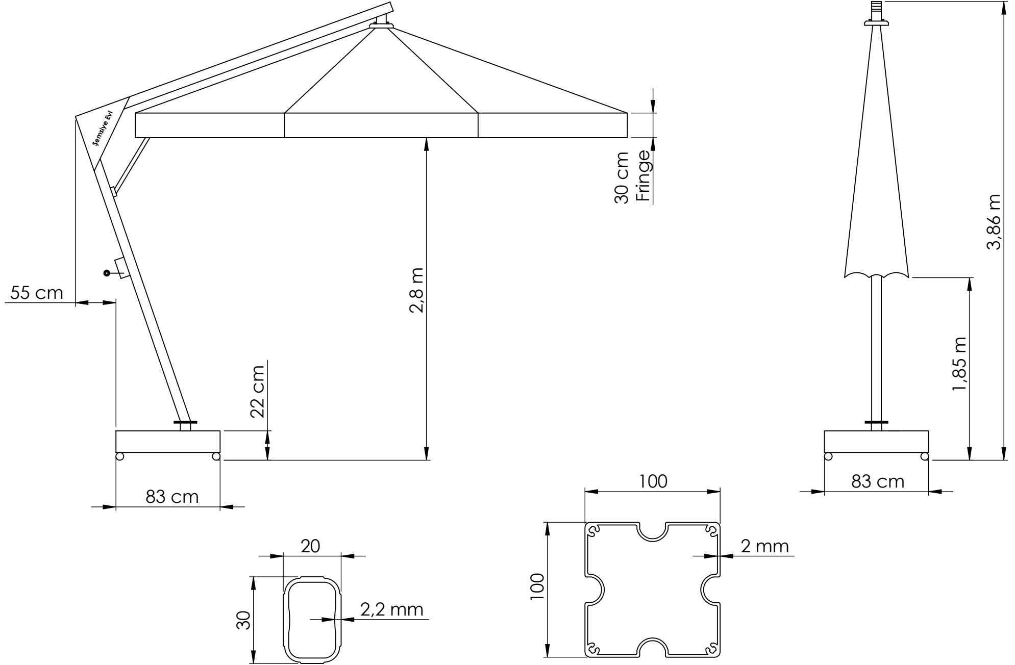
Profil / Ribs
